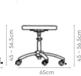
Revolving Stool (Without Back)
